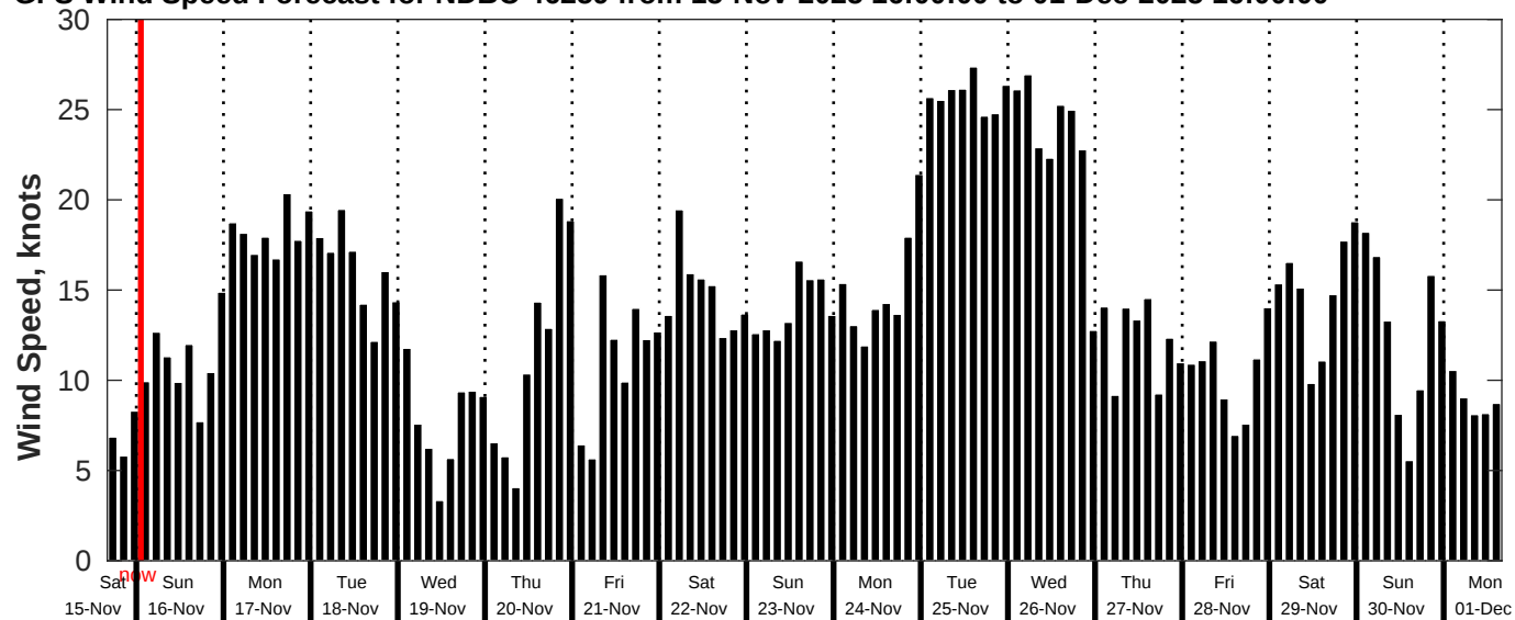
GFS Wind Speed Forecast for NDBC 46259 from 15-Nov-2025 16:00:00 to 01-Dec-2025 16:00:00
