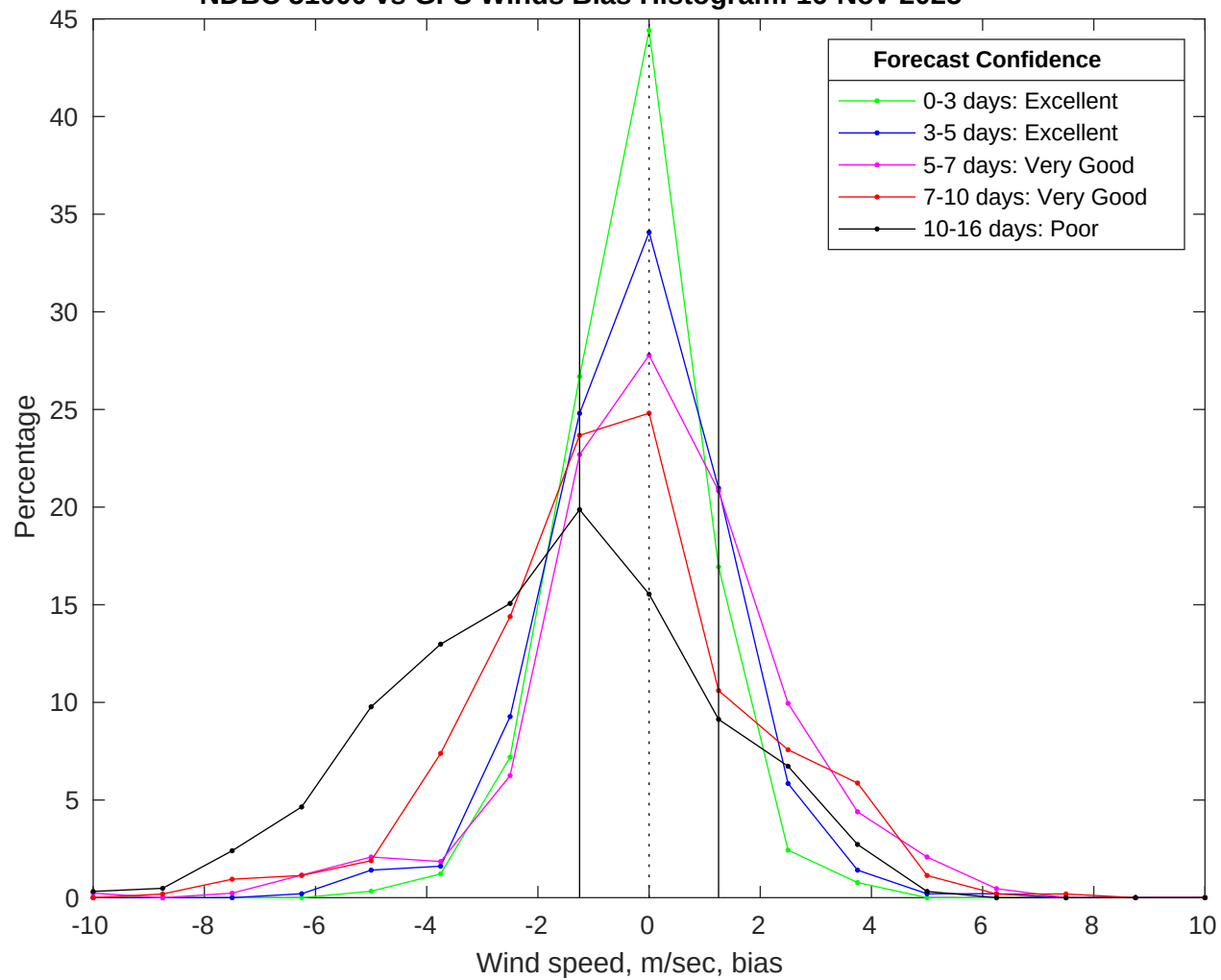
NDBC 51000 vs GFS Winds Bias Histogram: 16-Nov-2025
