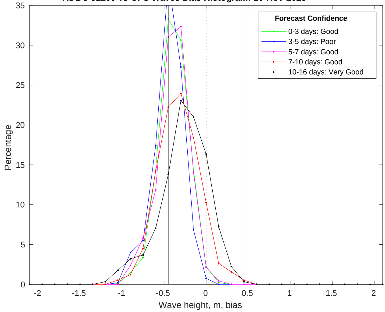
NDBC 51209 vs GFS Waves Bias Histogram: 16-Nov-2025
