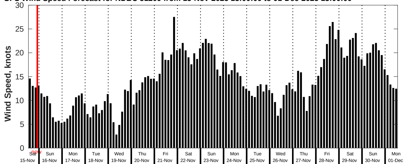
GFS Wind Speed Forecast for NDBC 51209 from 15-Nov-2025 13:00:00 to 01-Dec-2025 13:00:00
