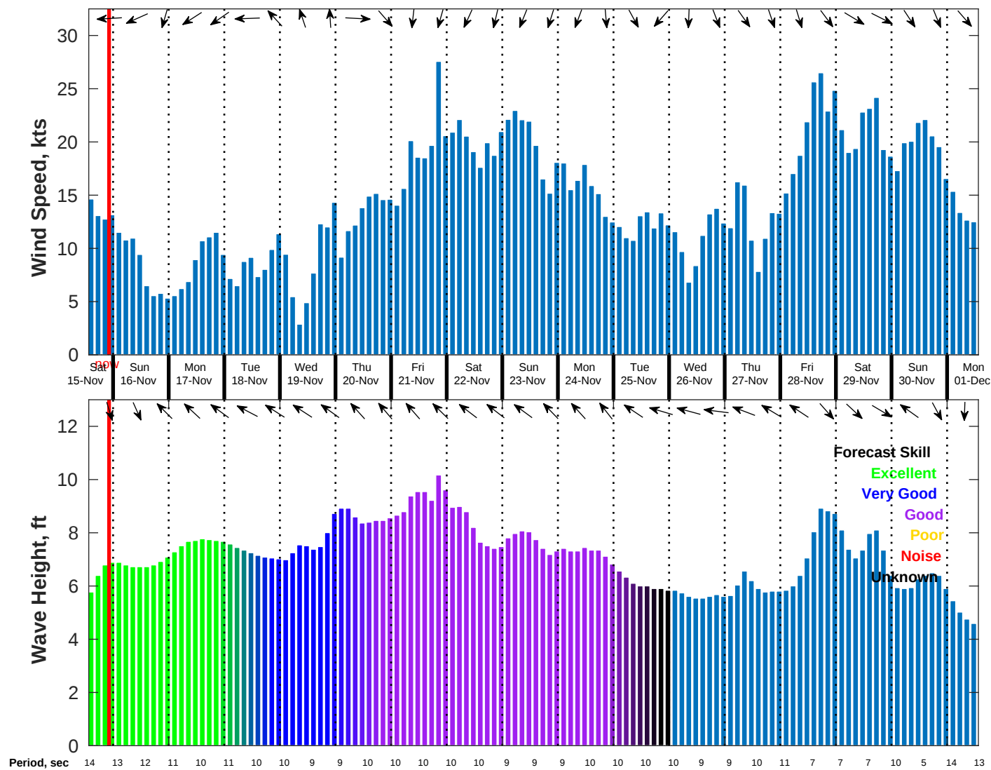
Wind & Wave Forecast for NDBC 51209 from 15-Nov-2025 13:00:00 to 01-Dec-2025 13:00:00
