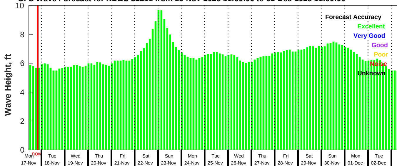
GFS Wave Forecast for NDBC 52211 from 16-Nov-2025 11:00:00 to 02-Dec-2025 11:00:00
