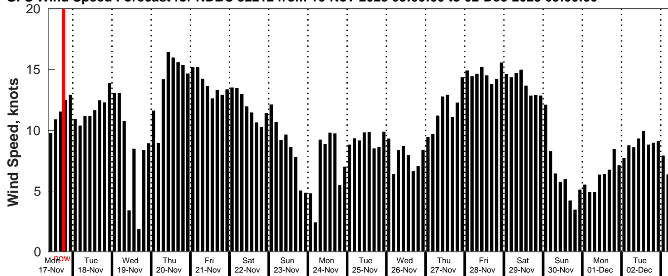
GFS Wind Speed Forecast for NDBC 52212 from 16-Nov-2025 09:00:00 to 02-Dec-2025 09:00:00
