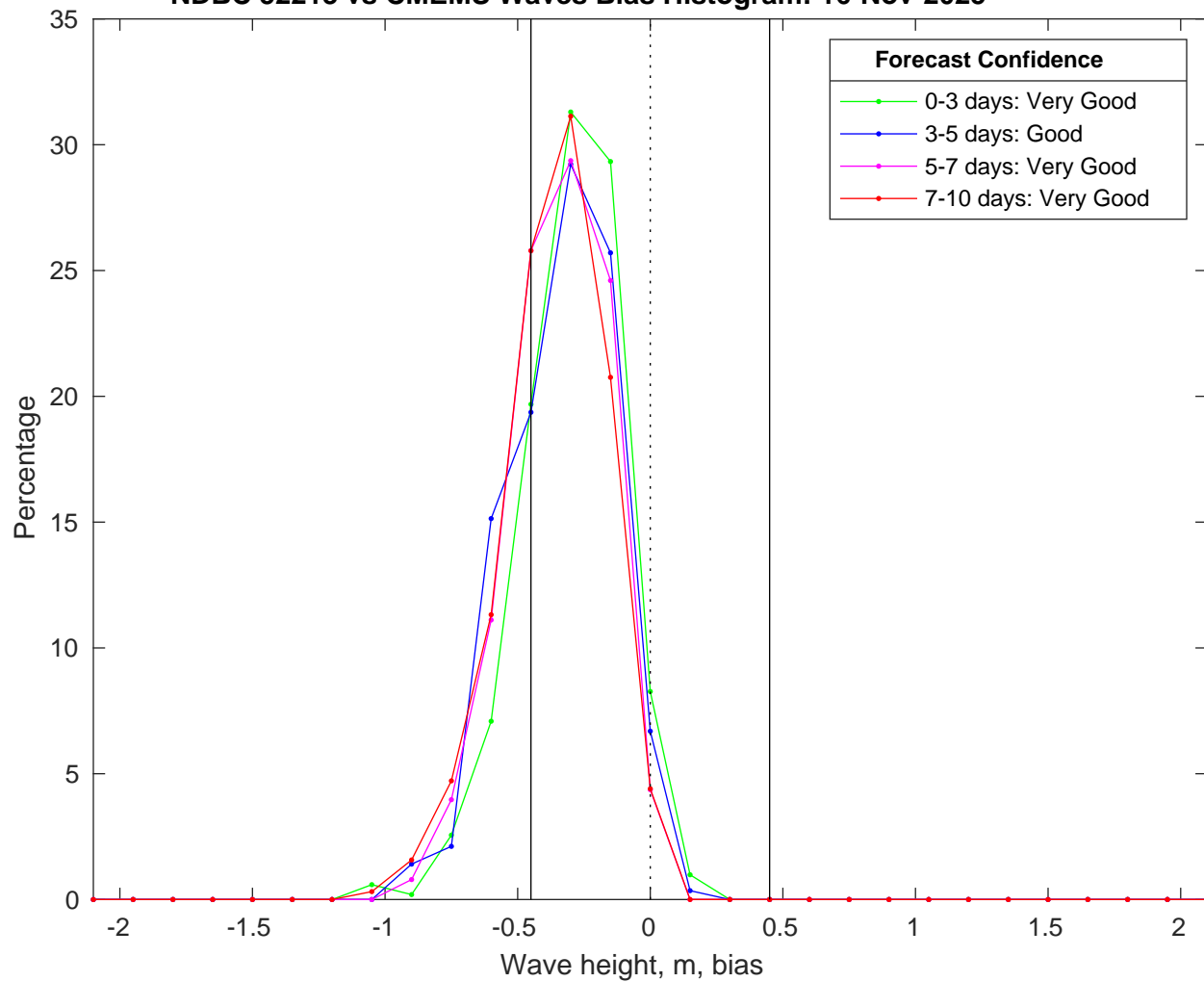
NDBC 52213 vs CMEMS Waves Bias Histogram: 16-Nov-2025
