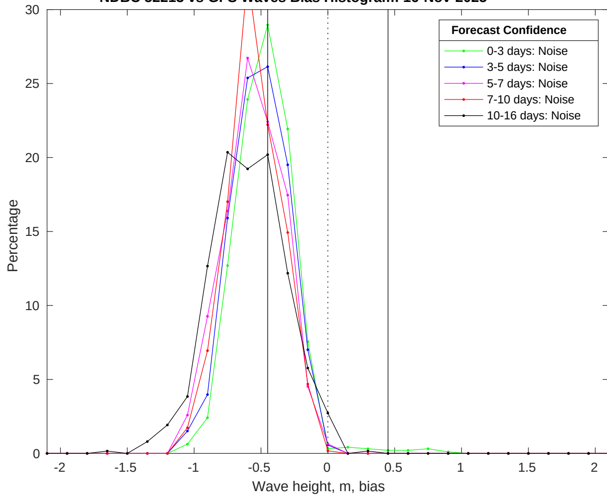
NDBC 52213 vs GFS Waves Bias Histogram: 16-Nov-2025
