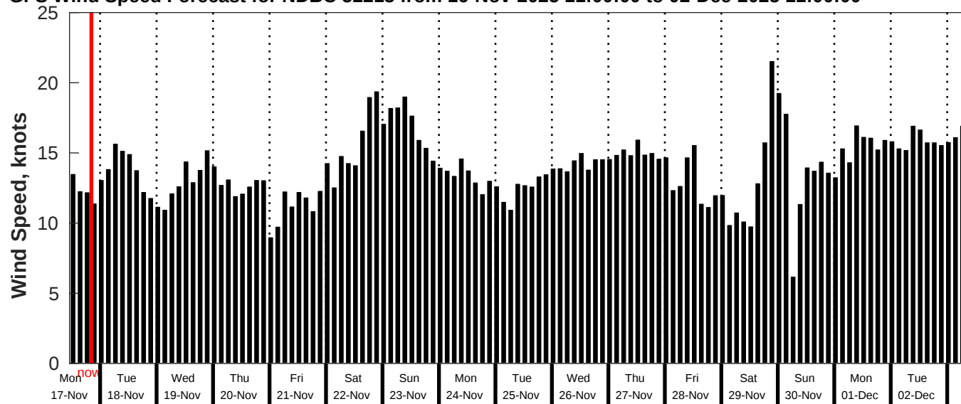
GFS Wind Speed Forecast for NDBC 52213 from 16-Nov-2025 11:00:00 to 02-Dec-2025 11:00:00
