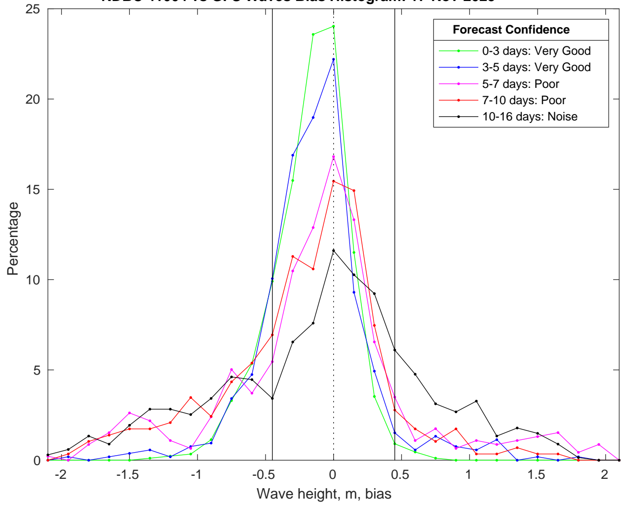
NDBC 41004 vs GFS Waves Bias Histogram: 17-Nov-2025
