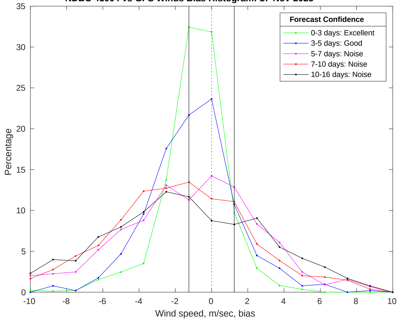
NDBC 41004 vs GFS Winds Bias Histogram: 17-Nov-2025
