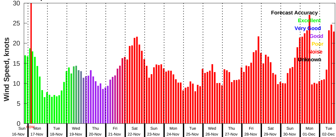
GFS Wind Speed Forecast for NDBC 41004 from 16-Nov-2025 19:00:00 to 02-Dec-2025 19:00:00
