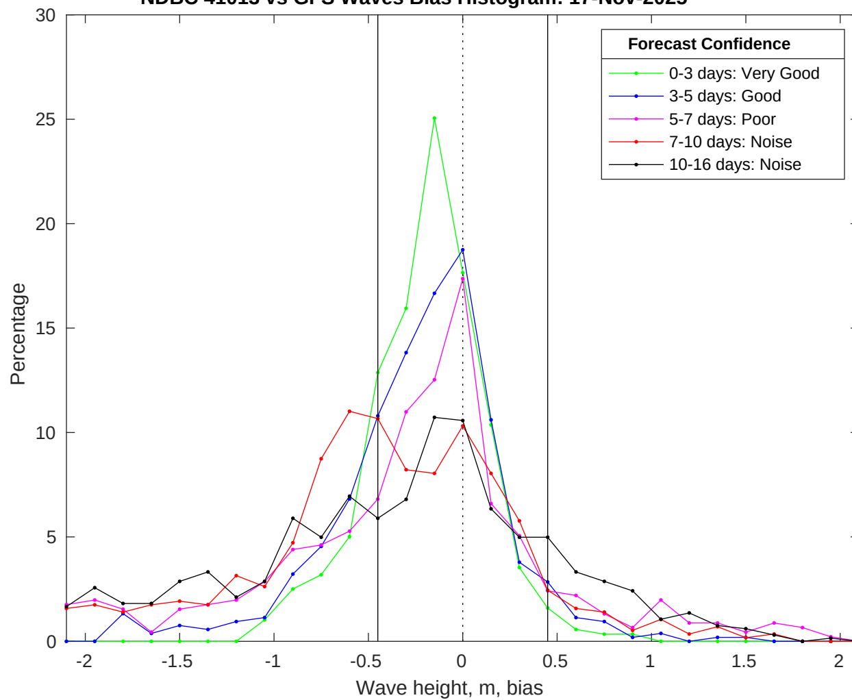
NDBC 41013 vs GFS Waves Bias Histogram: 17-Nov-2025
