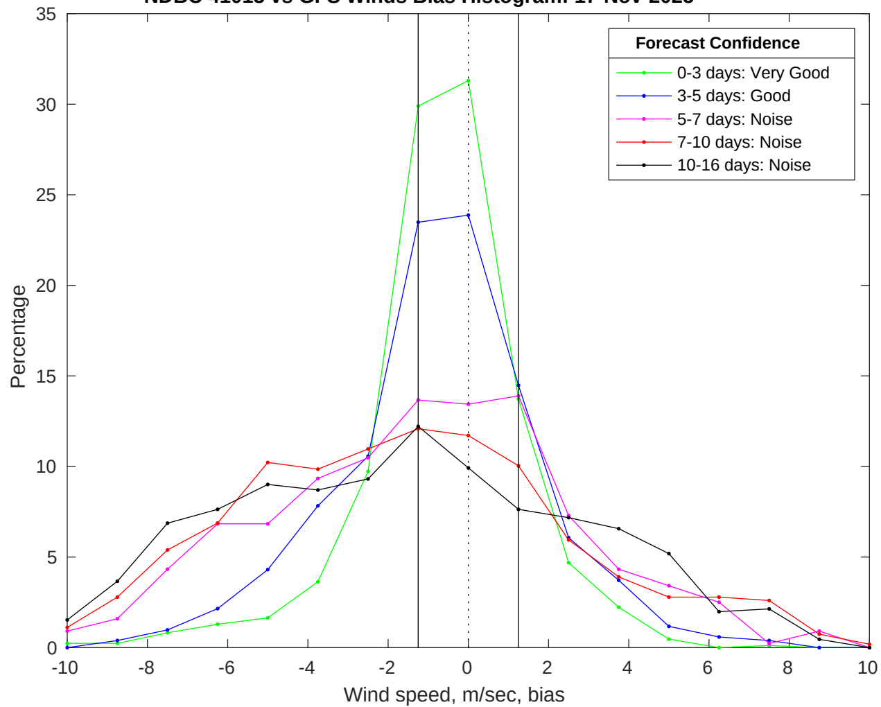
NDBC 41013 vs GFS Winds Bias Histogram: 17-Nov-2025
