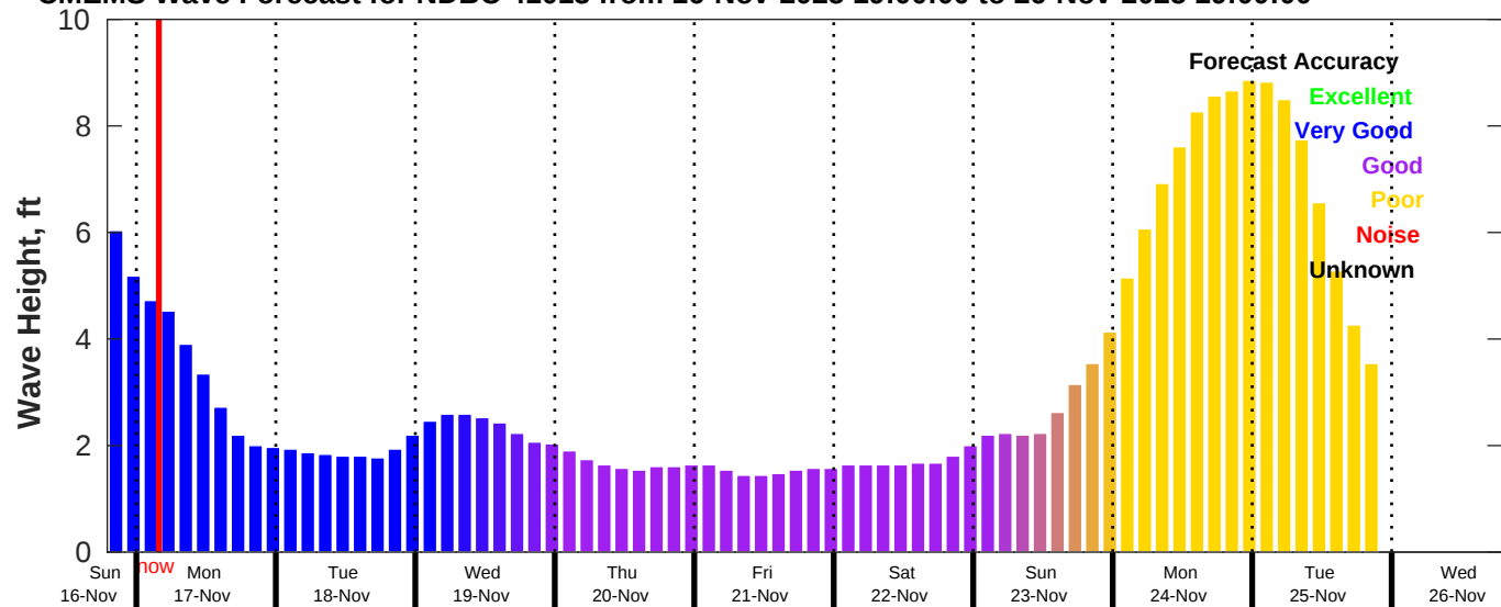
CMEMS Wave Forecast for NDBC 41013 from 16-Nov-2025 19:00:00 to 26-Nov-2025 19:00:00
