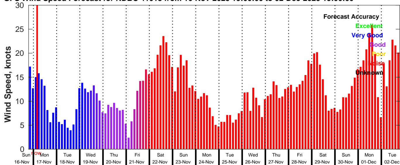
GFS Wind Speed Forecast for NDBC 41013 from 16-Nov-2025 19:00:00 to 02-Dec-2025 19:00:00
