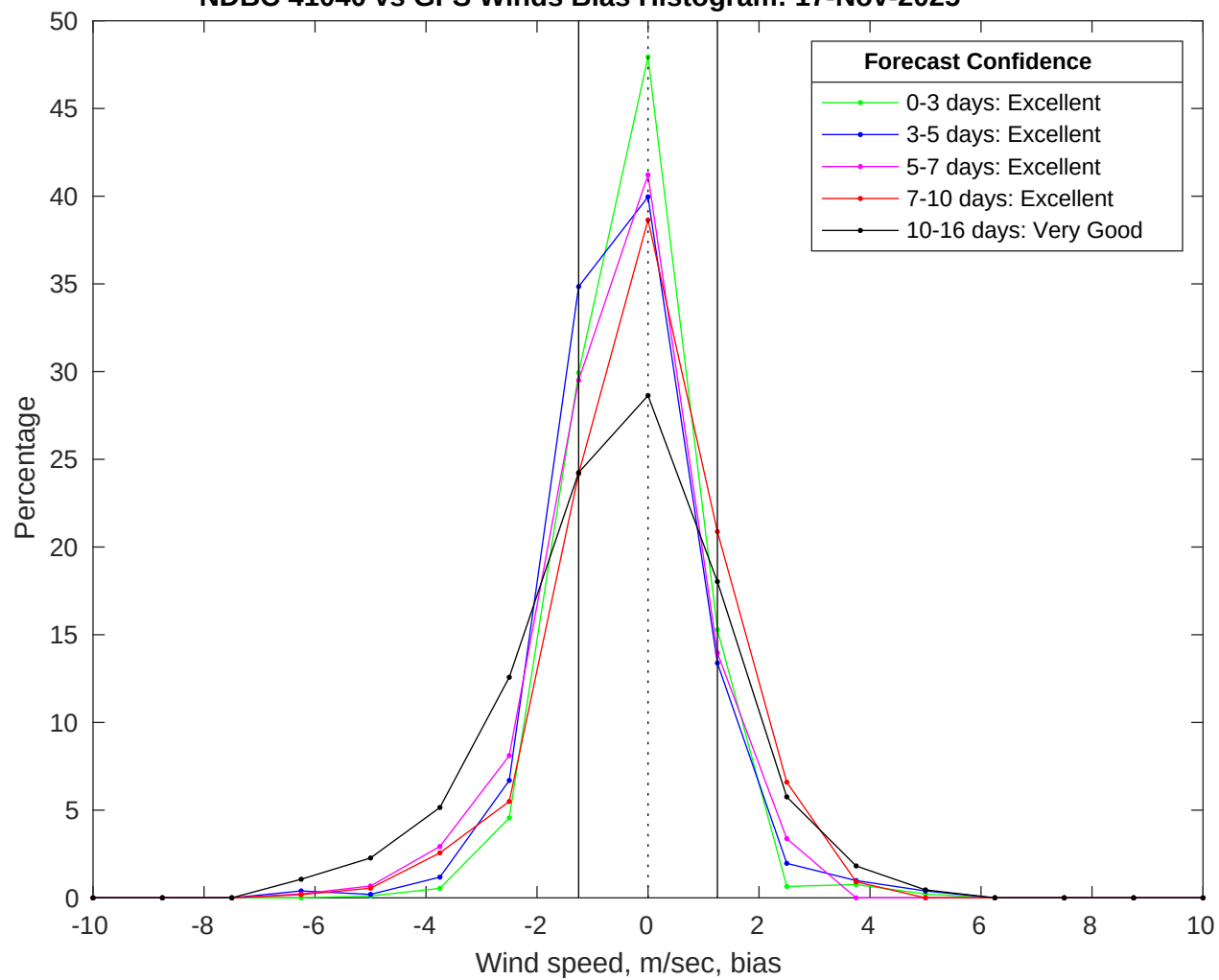
NDBC 41040 vs GFS Winds Bias Histogram: 17-Nov-2025
