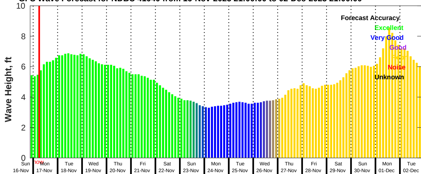
GFS Wave Forecast for NDBC 41040 from 16-Nov-2025 21:00:00 to 02-Dec-2025 21:00:00
