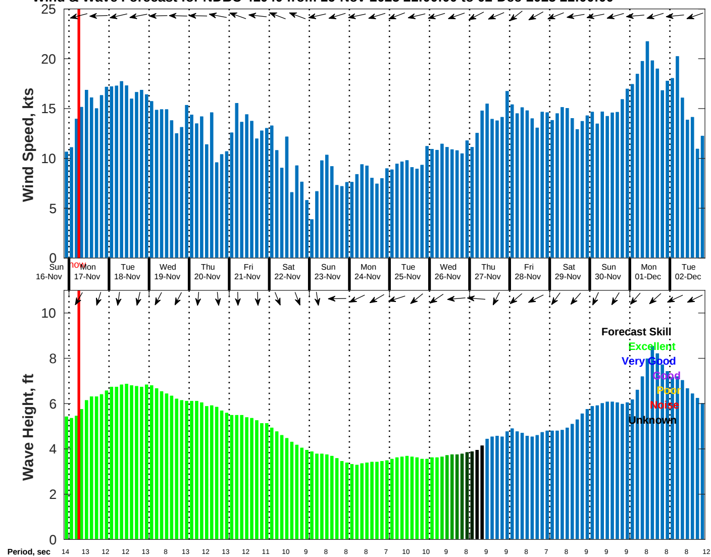
Wind & Wave Forecast for NDBC 41040 from 16-Nov-2025 21:00:00 to 02-Dec-2025 21:00:00
