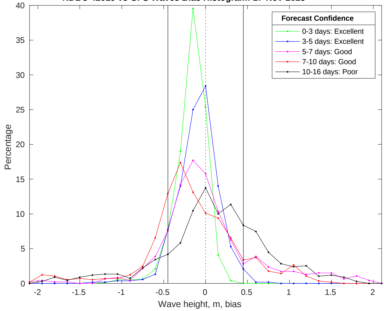
NDBC 42019 vs GFS Waves Bias Histogram: 17-Nov-2025
