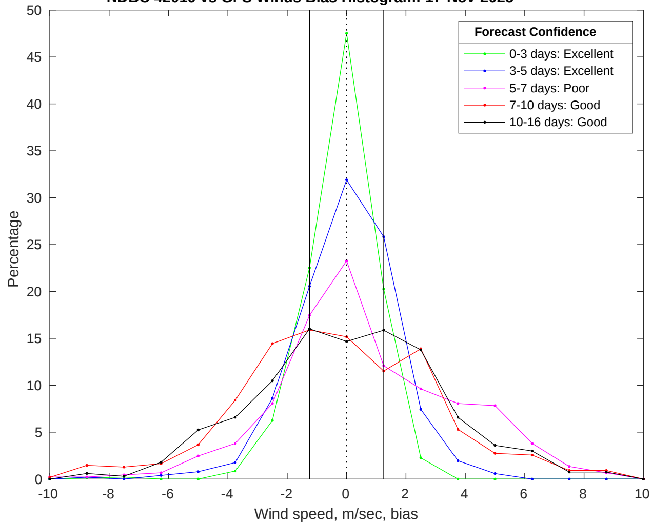
NDBC 42019 vs GFS Winds Bias Histogram: 17-Nov-2025
