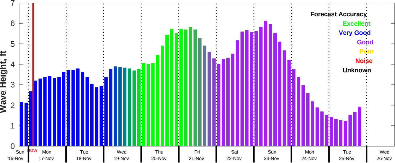
CMEMS Wave Forecast for NDBC 42019 from 16-Nov-2025 18:00:00 to 26-Nov-2025 18:00:00
