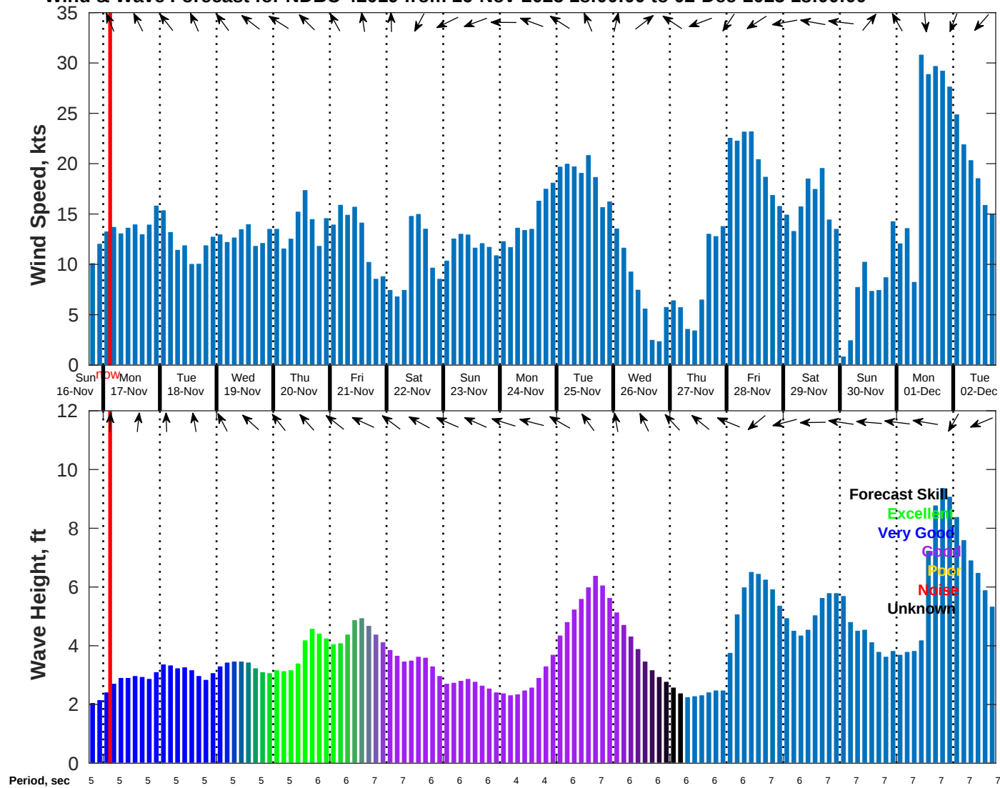
Wind & Wave Forecast for NDBC 42019 from 16-Nov-2025 18:00:00 to 02-Dec-2025 18:00:00
