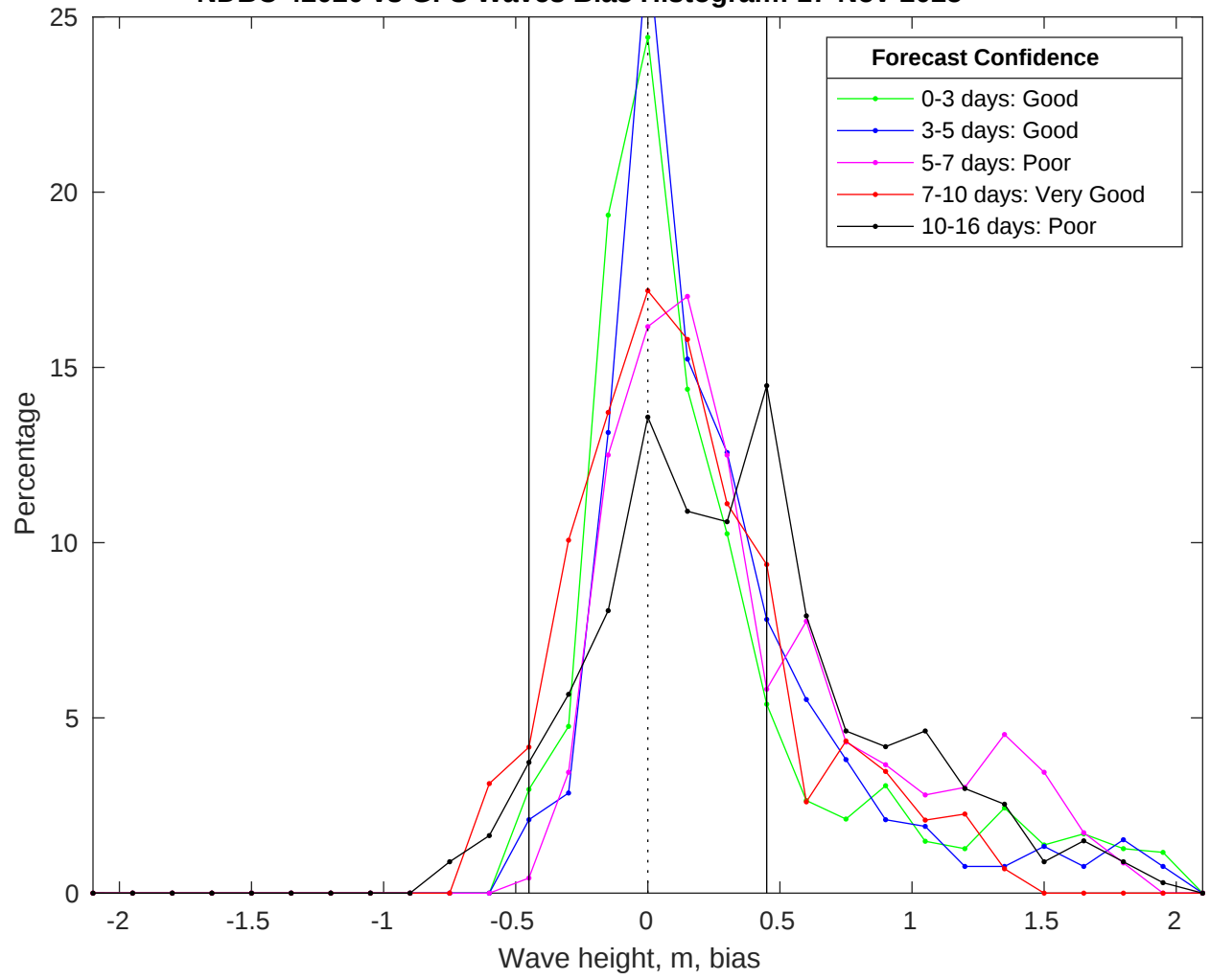
NDBC 42020 vs GFS Waves Bias Histogram: 17-Nov-2025
