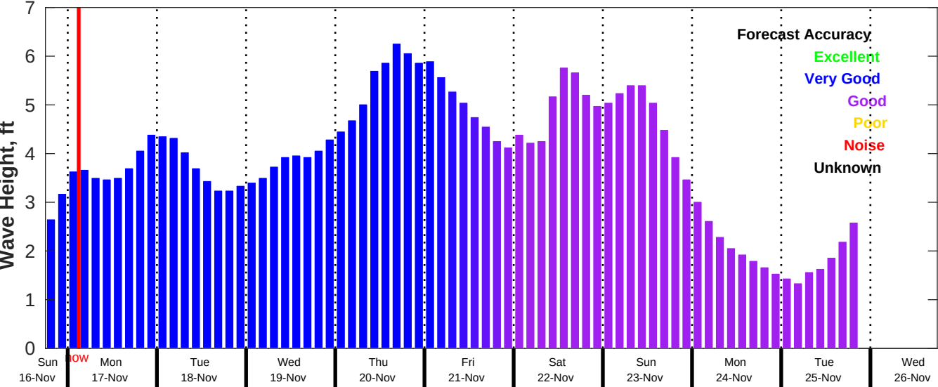
CMEMS Wave Forecast for NDBC 42020 from 16-Nov-2025 18:00:00 to 26-Nov-2025 18:00:00
