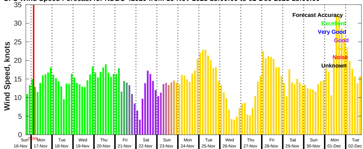
GFS Wind Speed Forecast for NDBC 42020 from 16-Nov-2025 18:00:00 to 02-Dec-2025 18:00:00
