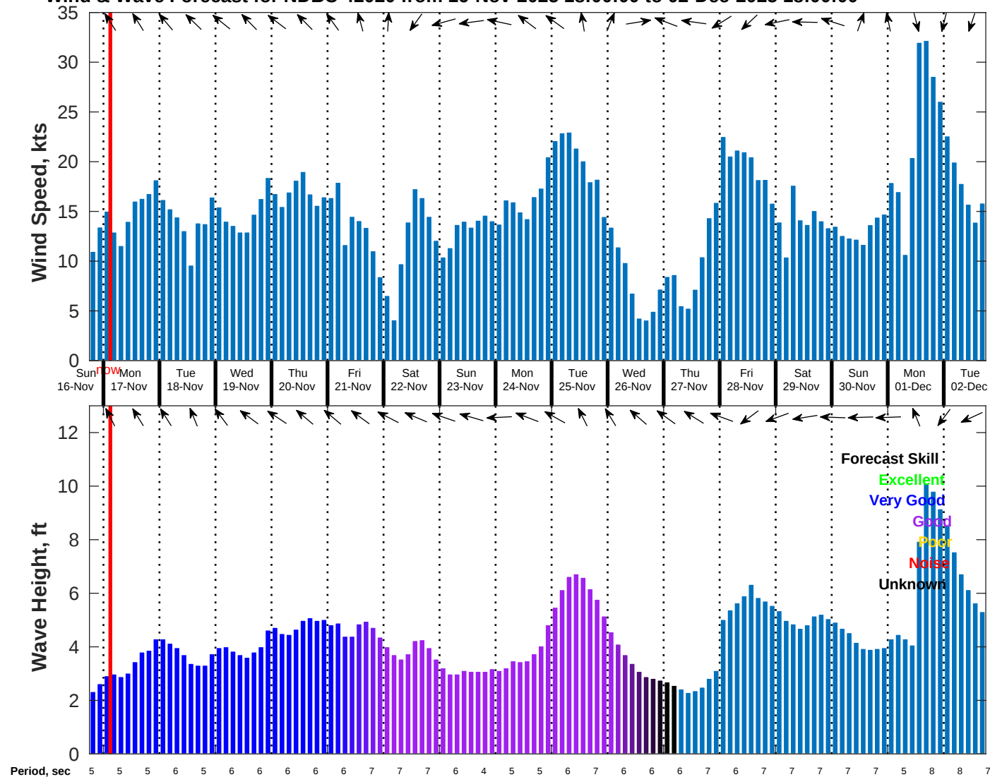
Wind & Wave Forecast for NDBC 42020 from 16-Nov-2025 18:00:00 to 02-Dec-2025 18:00:00
