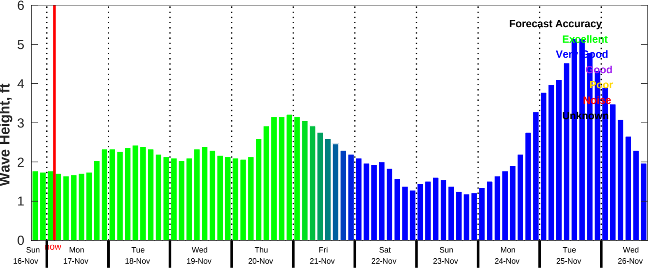
CMEMS Wave Forecast for NDBC 42035 from 16-Nov-2025 18:00:00 to 26-Nov-2025 18:00:00
