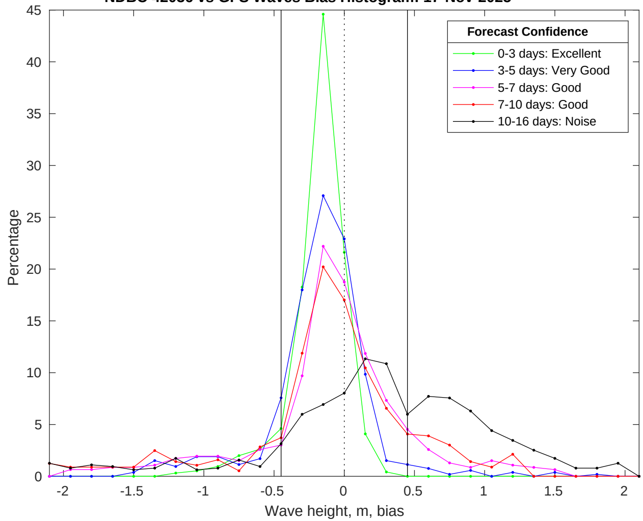
NDBC 42036 vs GFS Waves Bias Histogram: 17-Nov-2025
