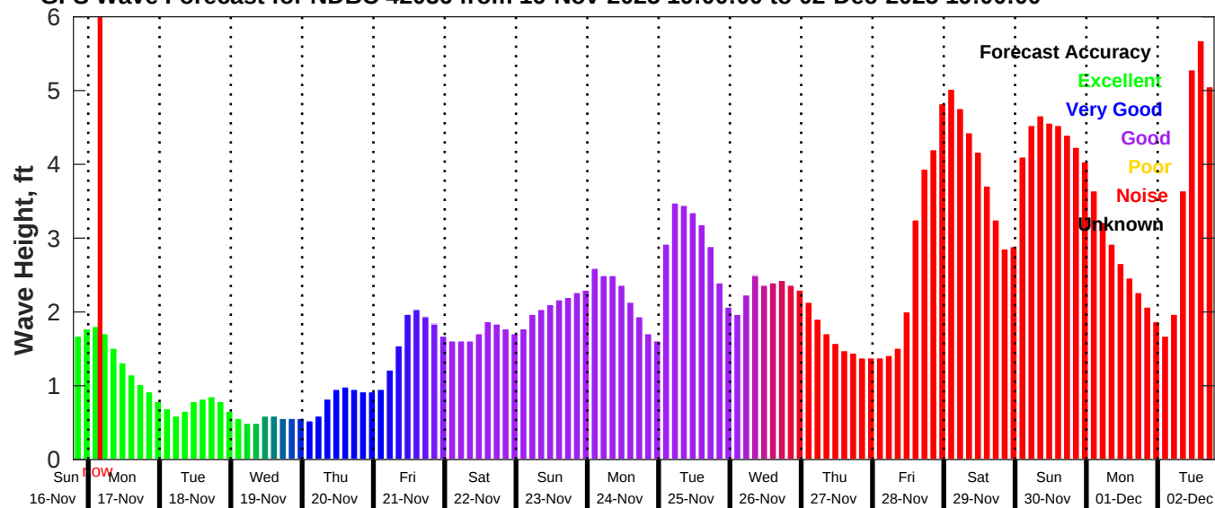
GFS Wave Forecast for NDBC 42036 from 16-Nov-2025 19:00:00 to 02-Dec-2025 19:00:00
