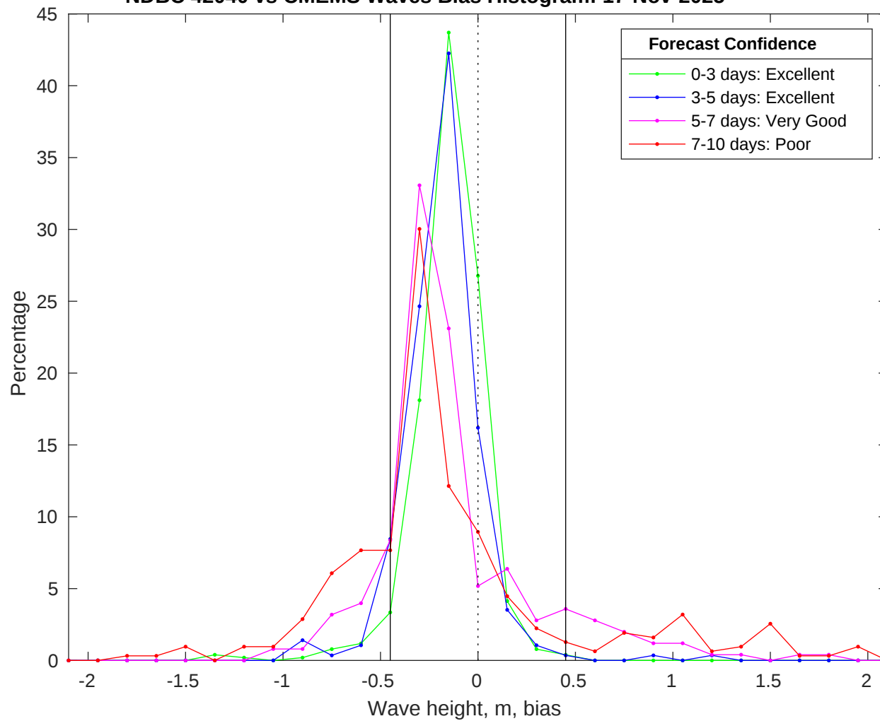
NDBC 42040 vs CMEMS Waves Bias Histogram: 17-Nov-2025
