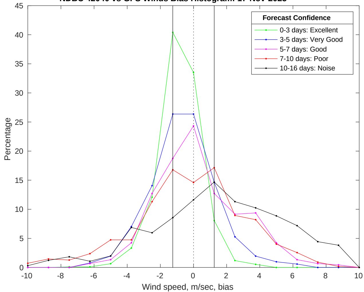
NDBC 42040 vs GFS Winds Bias Histogram: 17-Nov-2025
