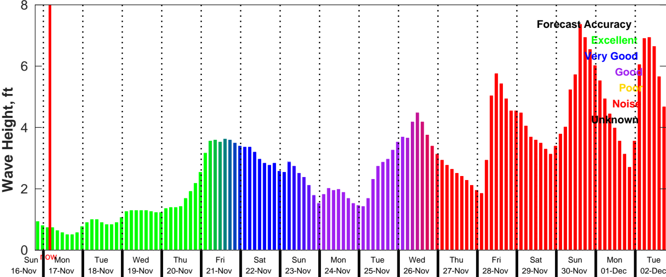
GFS Wave Forecast for NDBC 42040 from 16-Nov-2025 19:00:00 to 02-Dec-2025 19:00:00
