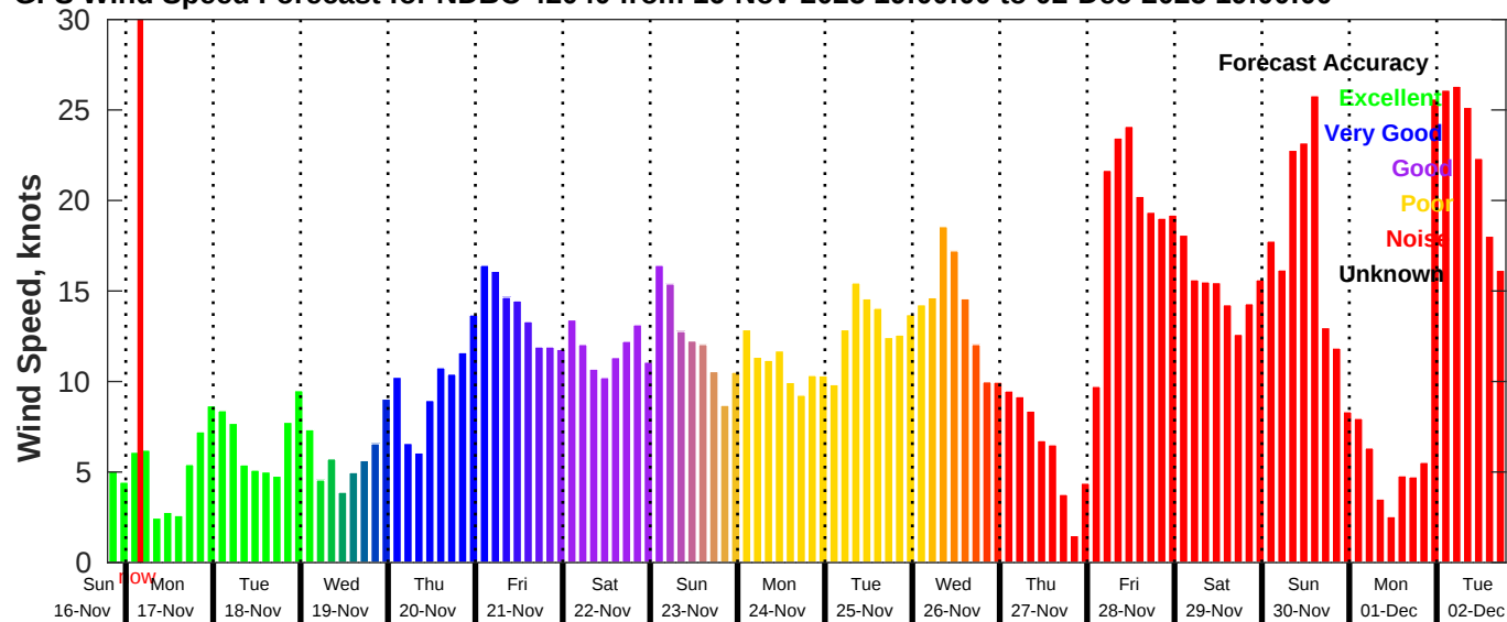
GFS Wind Speed Forecast for NDBC 42040 from 16-Nov-2025 19:00:00 to 02-Dec-2025 19:00:00
