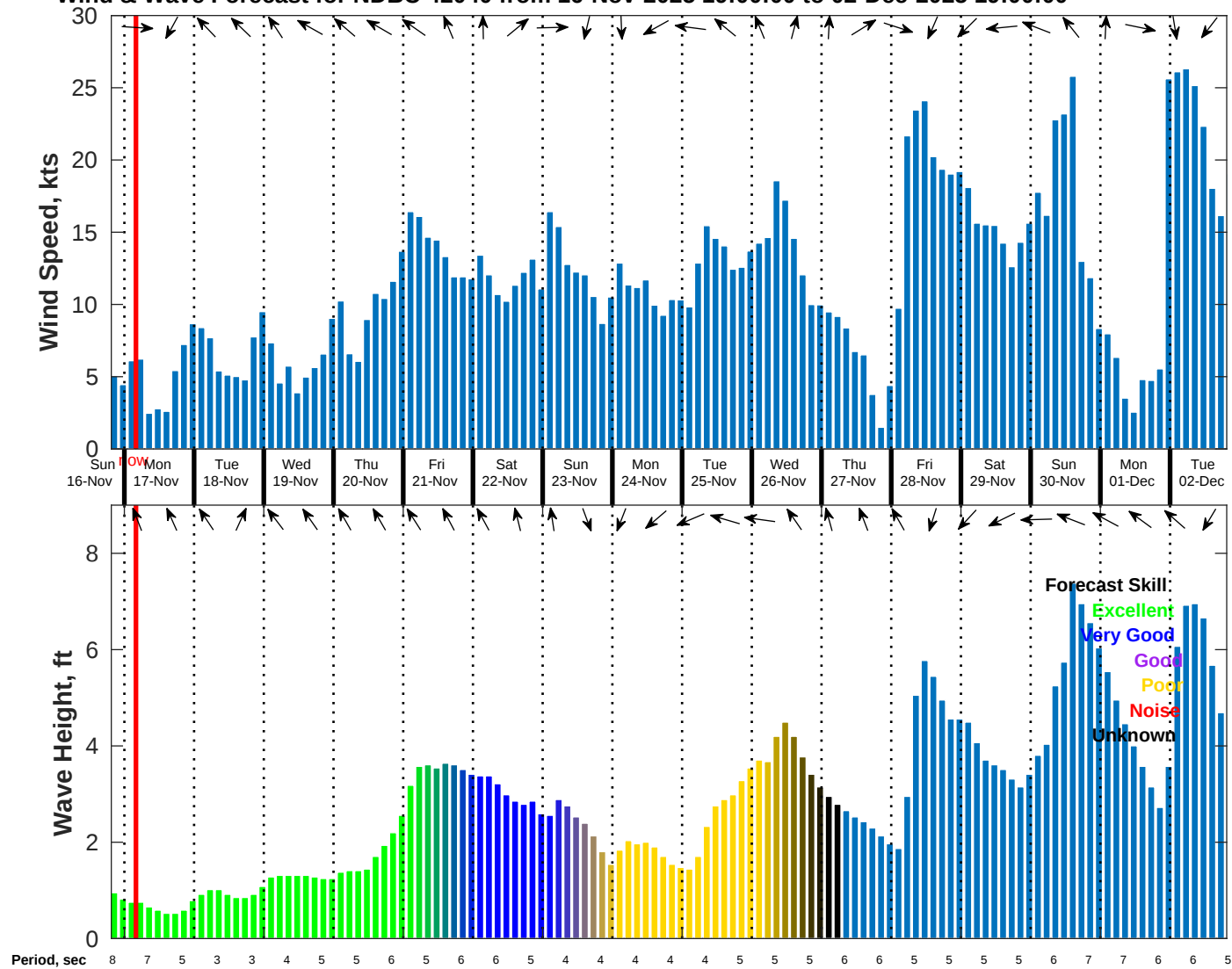
Wind & Wave Forecast for NDBC 42040 from 16-Nov-2025 19:00:00 to 02-Dec-2025 19:00:00
