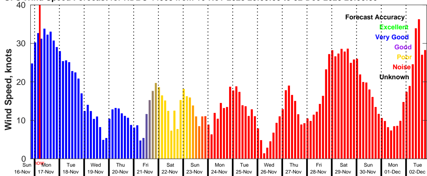
GFS Wind Speed Forecast for NDBC 44008 from 16-Nov-2025 20:00:00 to 02-Dec-2025 20:00:00
