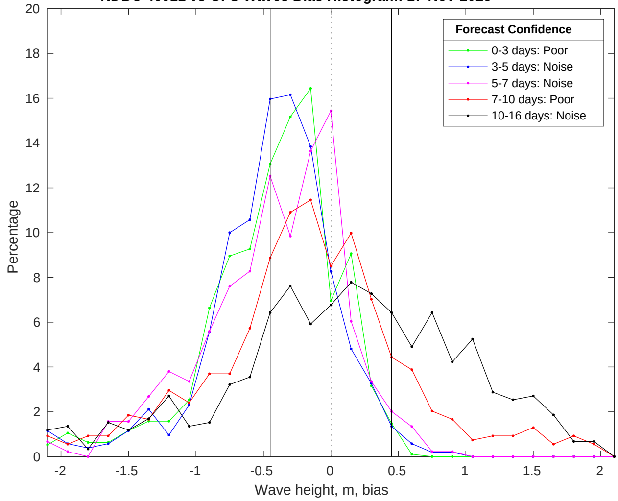
NDBC 46011 vs GFS Waves Bias Histogram: 17-Nov-2025
