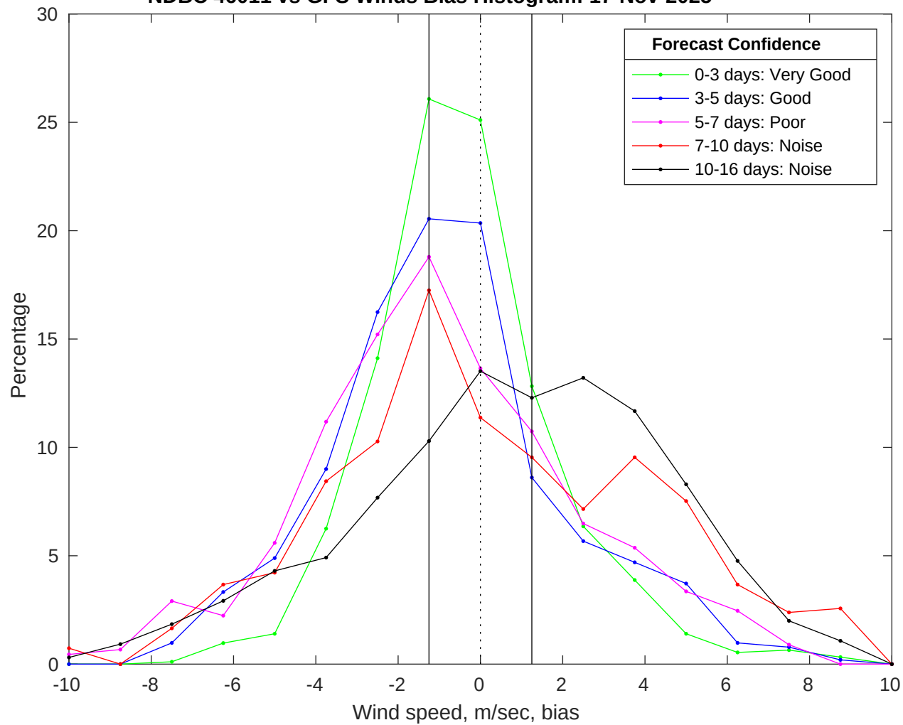
NDBC 46011 vs GFS Winds Bias Histogram: 17-Nov-2025
