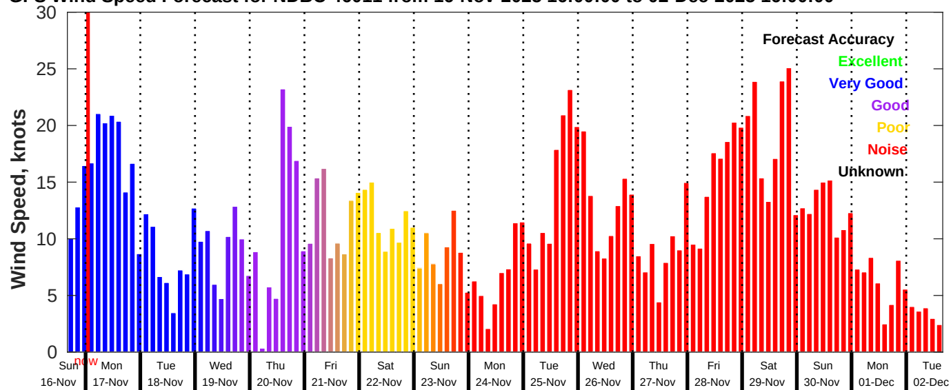
GFS Wind Speed Forecast for NDBC 46011 from 16-Nov-2025 16:00:00 to 02-Dec-2025 16:00:00
