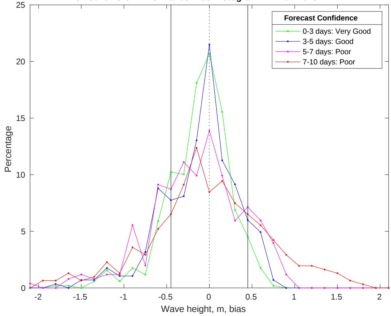
NDBC 46028 vs CMEMS Waves Bias Histogram: 17-Nov-2025
