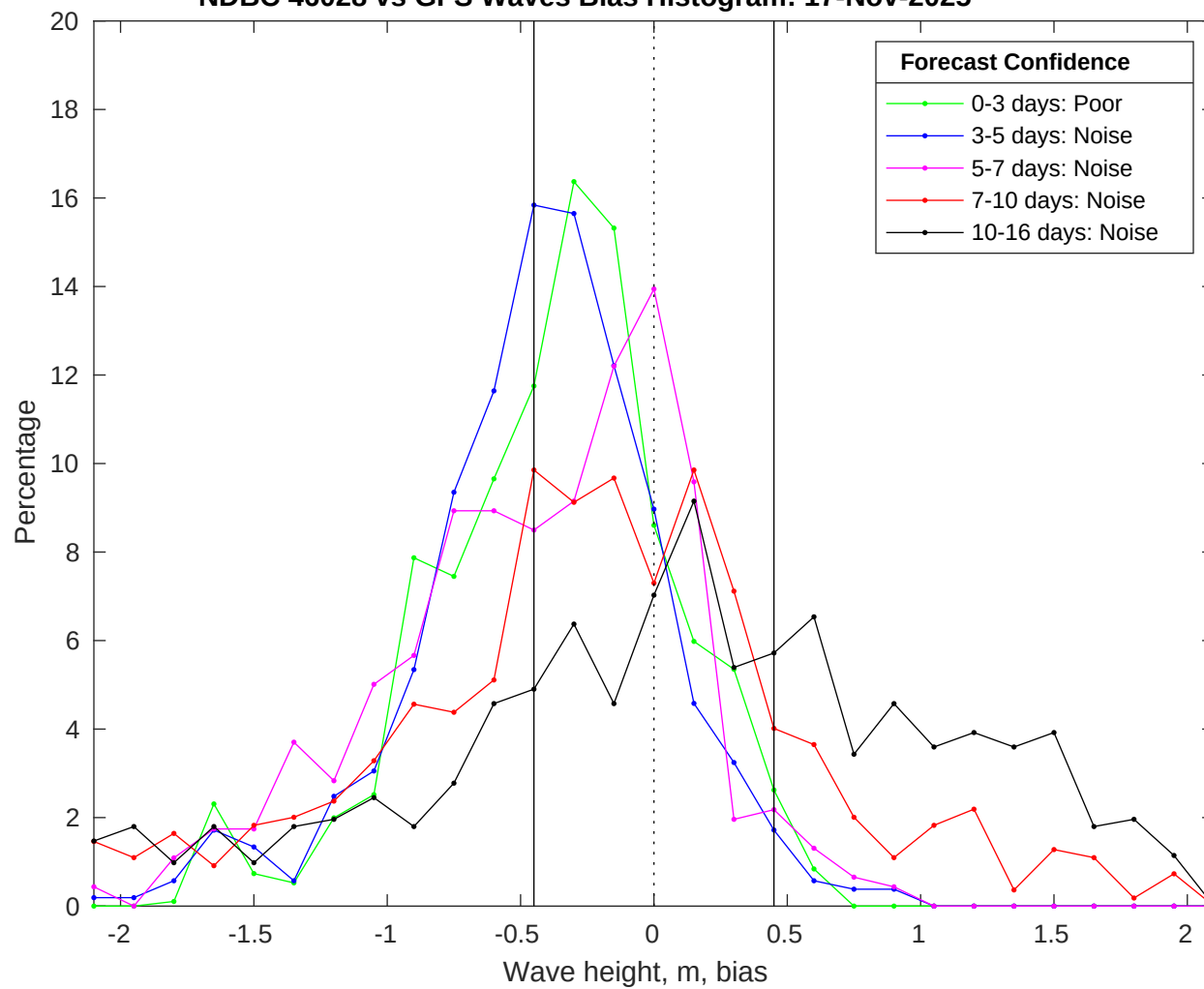
NDBC 46028 vs GFS Waves Bias Histogram: 17-Nov-2025
