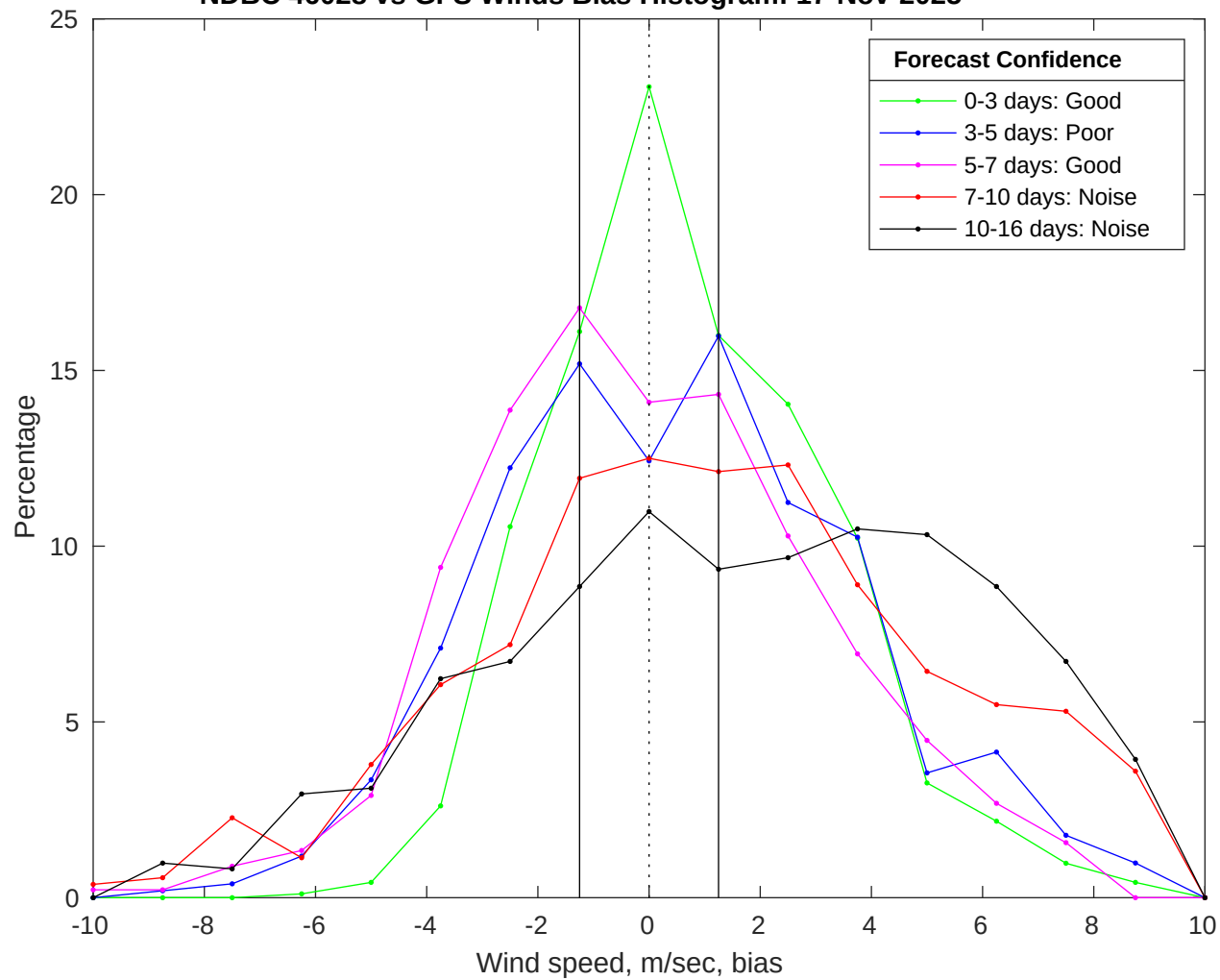
NDBC 46028 vs GFS Winds Bias Histogram: 17-Nov-2025
