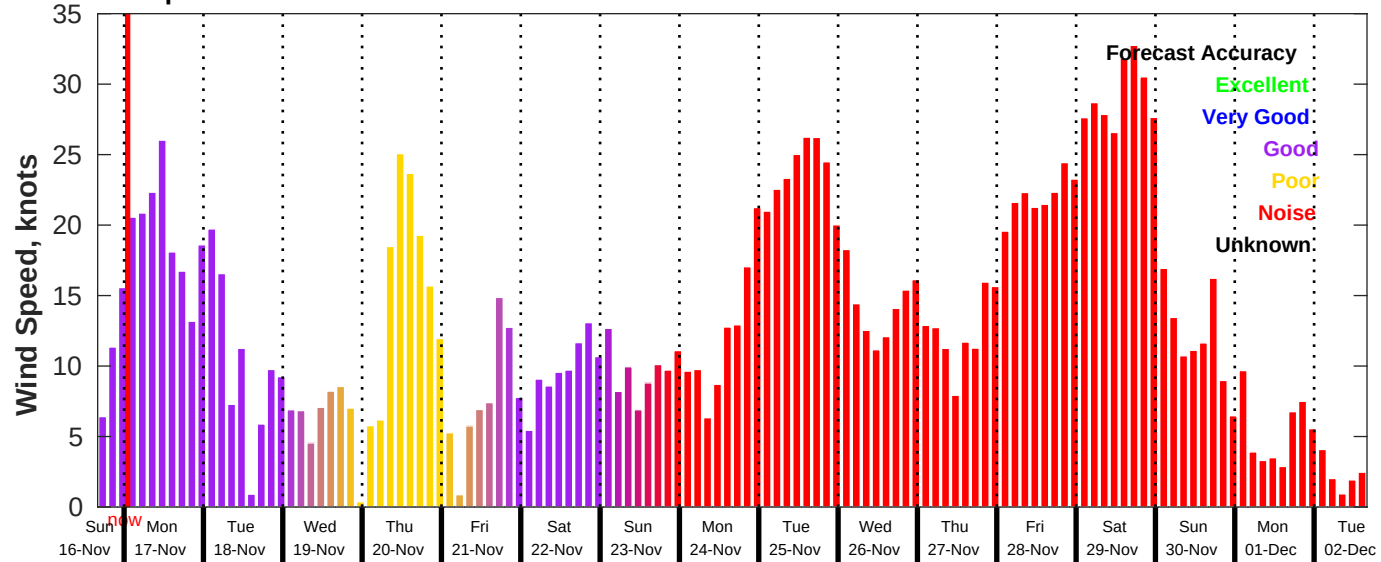
GFS Wind Speed Forecast for NDBC 46028 from 16-Nov-2025 16:00:00 to 02-Dec-2025 16:00:00
