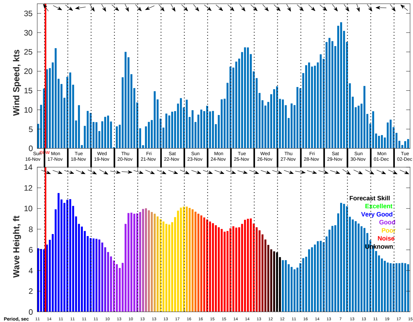
Wind & Wave Forecast for NDBC 46028 from 16-Nov-2025 16:00:00 to 02-Dec-2025 16:00:00
