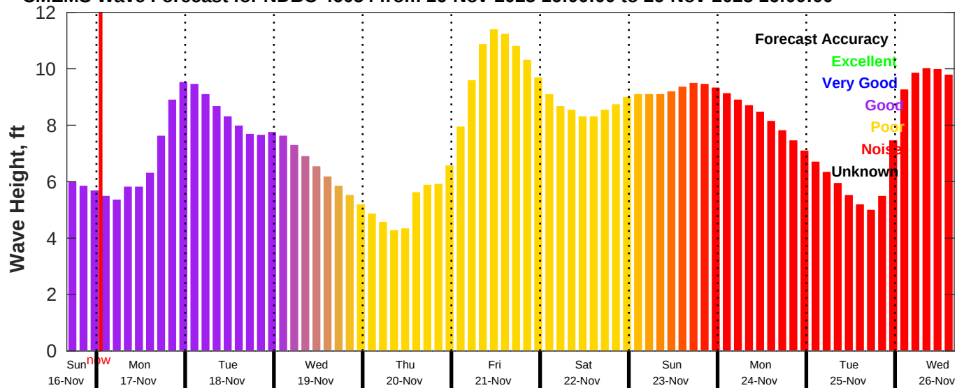
CMEMS Wave Forecast for NDBC 46054 from 16-Nov-2025 16:00:00 to 26-Nov-2025 16:00:00
