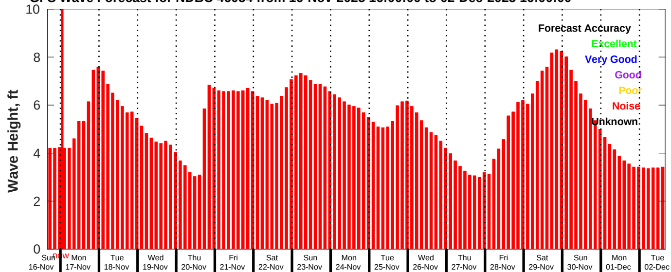
GFS Wave Forecast for NDBC 46054 from 16-Nov-2025 16:00:00 to 02-Dec-2025 16:00:00
