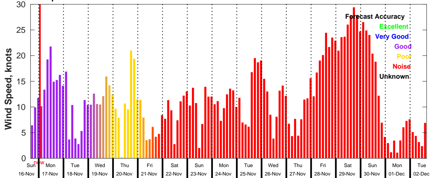
GFS Wind Speed Forecast for NDBC 46054 from 16-Nov-2025 16:00:00 to 02-Dec-2025 16:00:00
