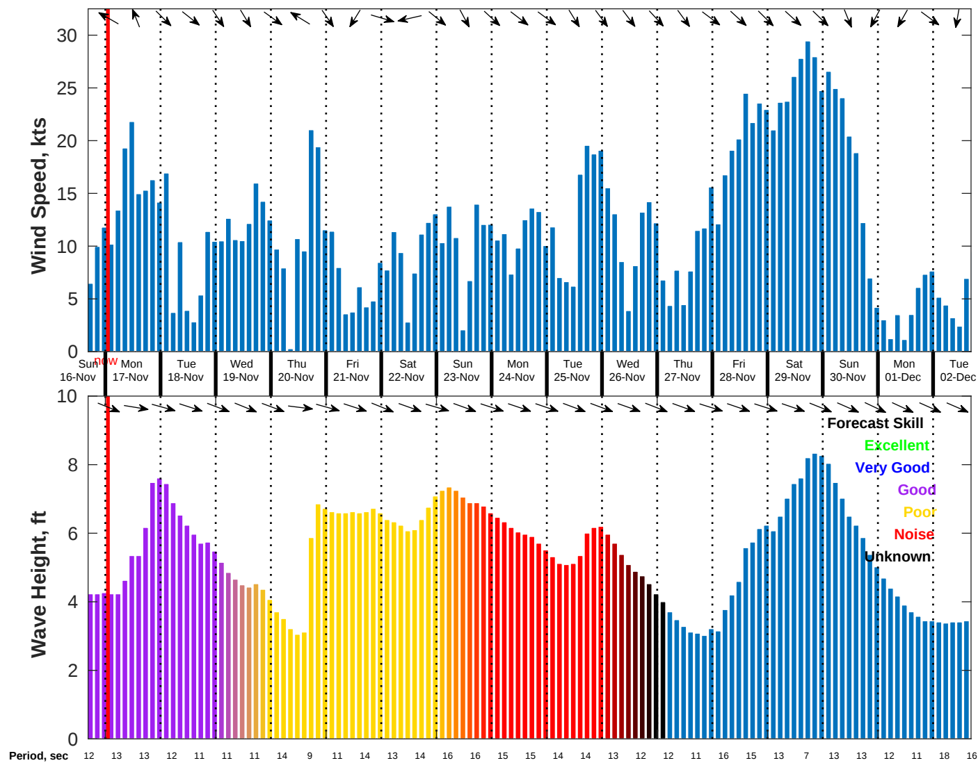
Wind & Wave Forecast for NDBC 46054 from 16-Nov-2025 16:00:00 to 02-Dec-2025 16:00:00
