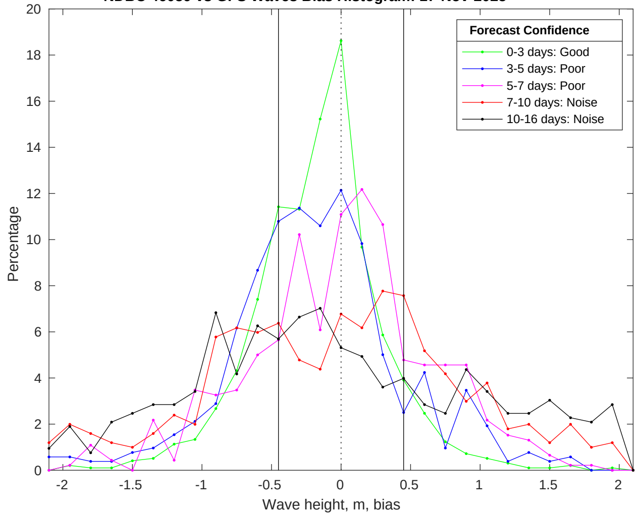
NDBC 46059 vs GFS Waves Bias Histogram: 17-Nov-2025
